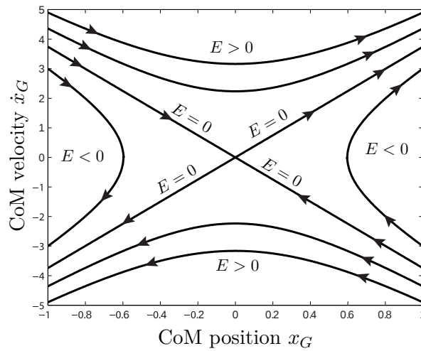
Figure 3-4: Phase portrait for the CoM of the Linear Inverted Pendulum Model. The CoP location is positioned at (0,0) . For E_{LIPM} > 0 , the CoM moves over the CoP. For E_{LIPM} < 0 moves to the CoM but moves back before it reaches the CoP. For E_{LIPM} = 0 the CoM comes to a stop over the CoP.
