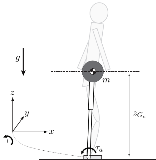
Figure 3-3: The LIPM consists of a point mass m and a massless telescopic leg. Ankle torque \tau_a can be applied at the base of the pendulum. The equation of motion of this model is linearised by constraining the CoM to fixed height z_{G_c} . The LIPM therefore simplifies the dynamics of the humanoid robot and can be used to derive an analytical solution for the ICP. The CoP is a point on the ground that indicates the amount of ankle torque applied. This point can be used to control the location of the ICP.
