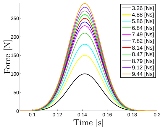
Figure 7-3: Disturbances applied in this simulation. The disturbances are applied to the CoM of the upper pendulum. The disturbance are generated by a Gaussian function and have the same time span and shape but vary in peak force. The applied impulse is calculated by the integral of the applied force over time and used as a measure for the disturbance.
