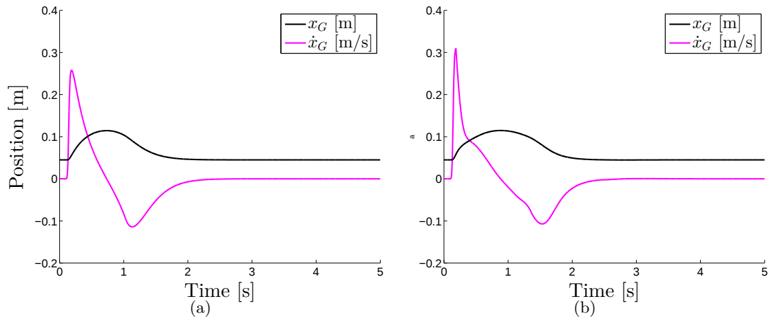
Figure 7-6: CoM position x_{CoM} and velocity \dot{x}_{CoM} for the ankle strategy (a) and the hip-ankle strategy (b). A large increase of CoM velocity is caused by the impulsive disturbance.
