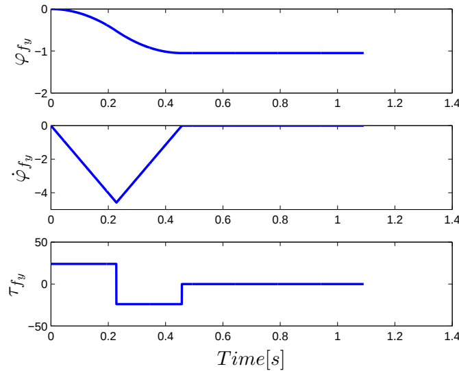
Figure 5-7: Flywheel response for a typical bang-bang hip-ankle strategy control action. The upper graph gives the flywheel angle \varphi_{f_y} over time, the flywheel velocity \dot{\varphi}_{f_y} is given by the middle graph. The bang-bang torque \tau_{f_y} profile is given by the lowest graph.
